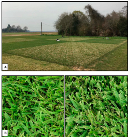
Fig. 1. Images showing St. Augustinegrass plots (A) exhibiting enhanced green color when mown with the autonomous mower in Mar 2019, and (B) quality of cut comparison between autonomous mower (left) vs conventional mulching mower (right) in Oct 2018.
